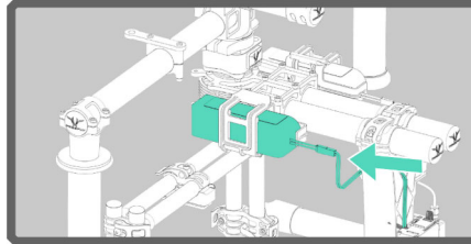
3. Ensure the MöVI power switch is set to "off" and plug the battery into the power input connector on the MöVI. Note: The battery and input connector are keyed. Do not force the battery and input connector together.
