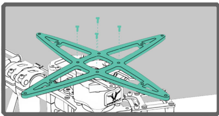
3. Attach the Octo Suspension Plate using the provided M3x10 Socket Head Cap Screws.
