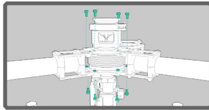
2. Attach the left and right landing gear legs and tubes to M10 using the provided M3x8 Socket Head Cap Screws.
